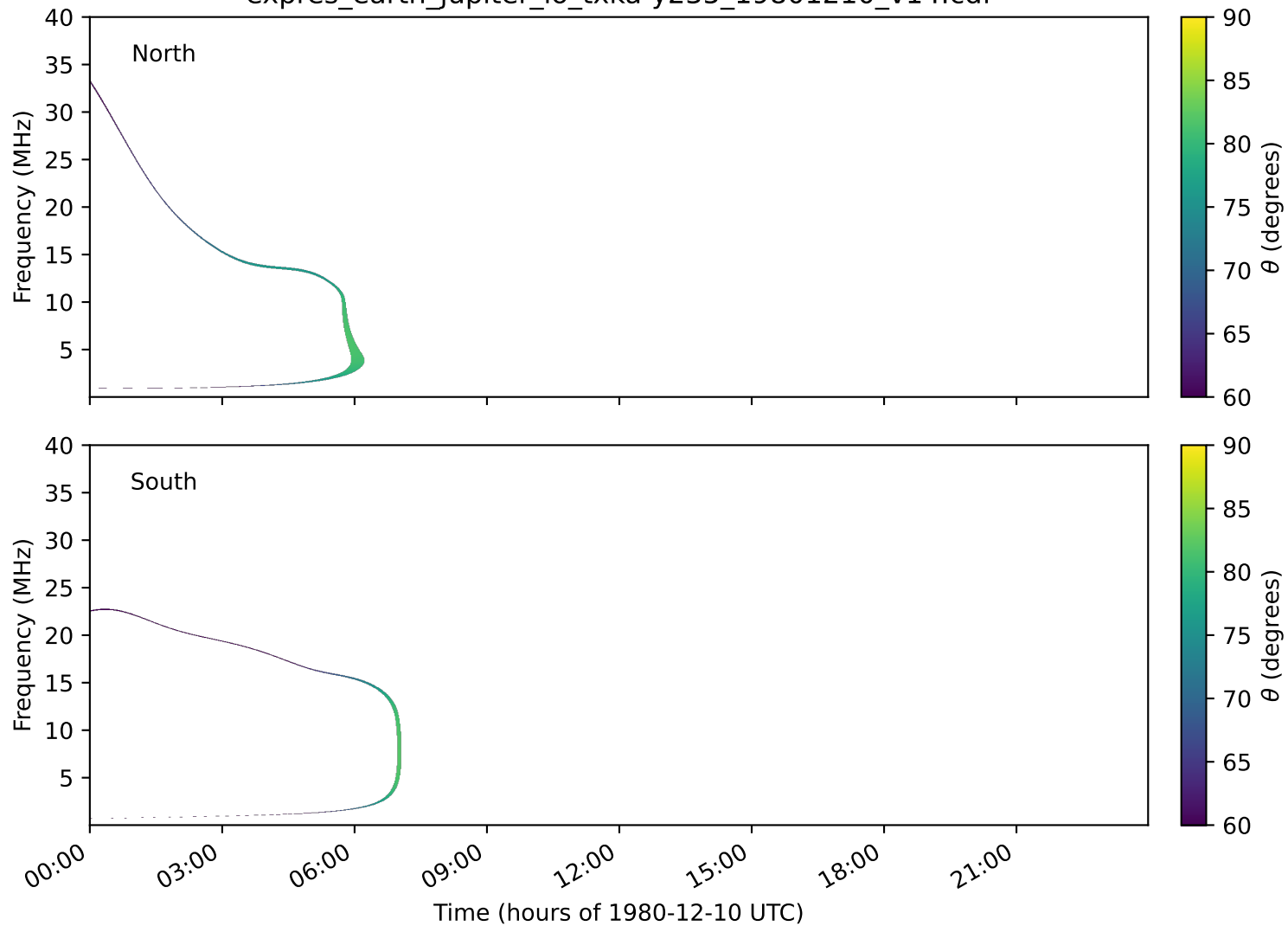
expres_earth_jupiter_io_txka-y235_19801210_v14.cdf
