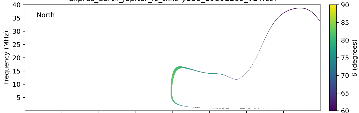
expres_earth_jupiter_io_txka-y235_19801209_v14.cdf
