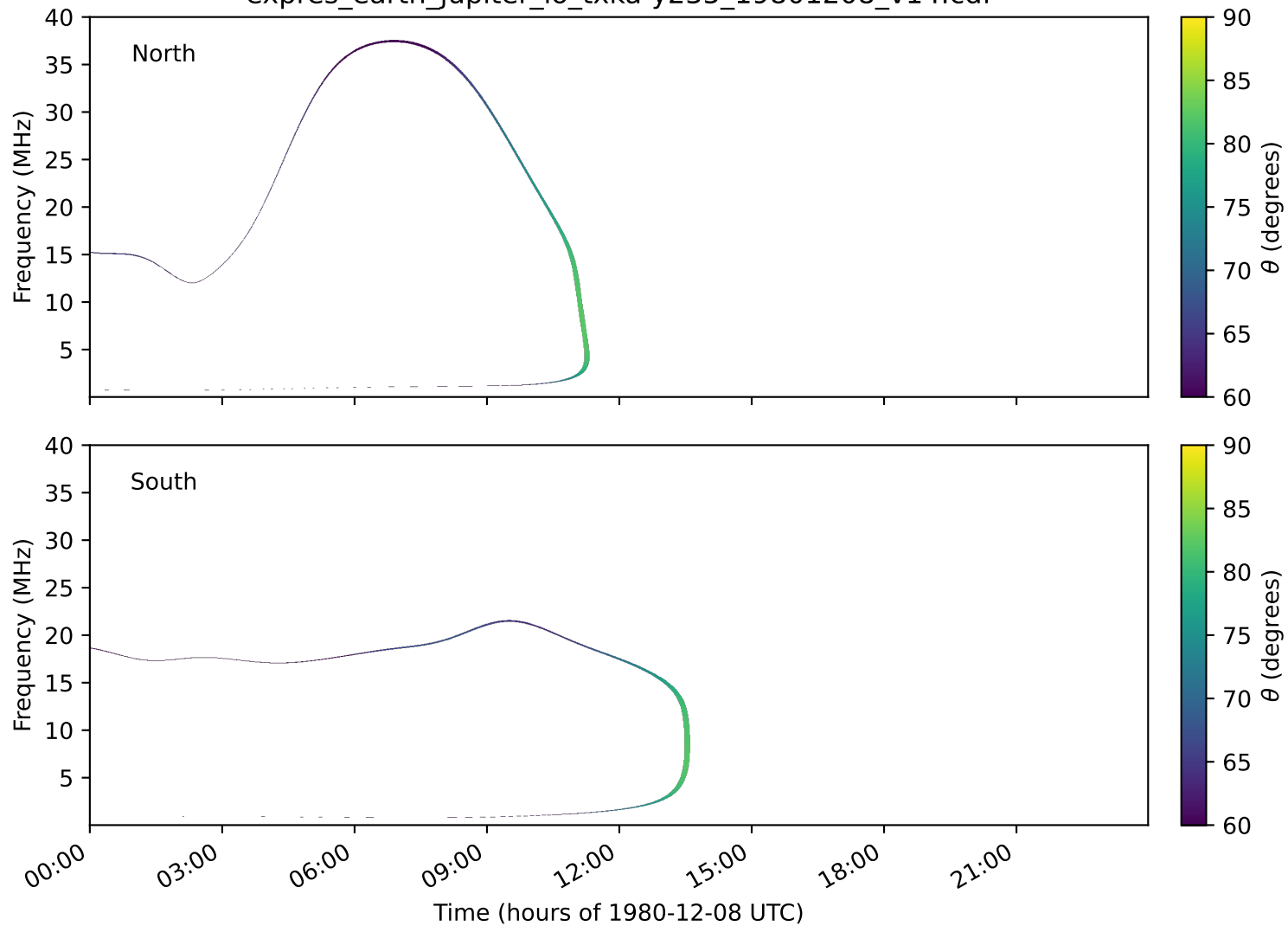
expres_earth_jupiter_io_txka-y235_19801208_v14.cdf
