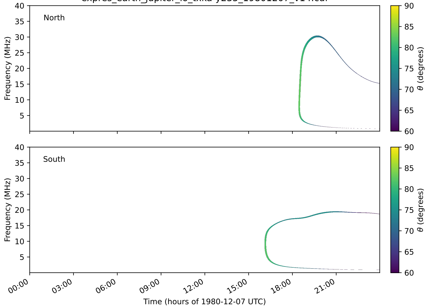
expres_earth_jupiter_io_txka-y235_19801207_v14.cdf
