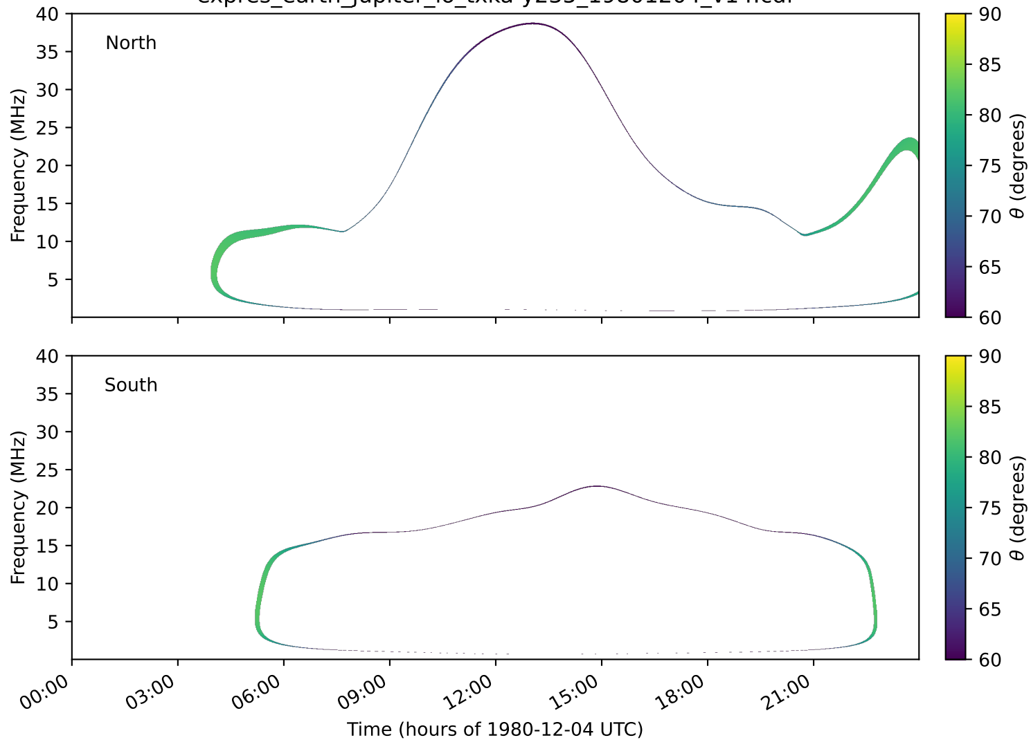
expres_earth_jupiter_io_txka-y235_19801204_v14.cdf
