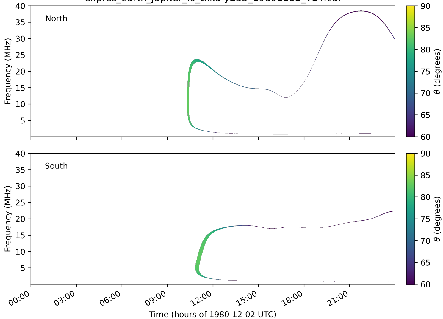
expres_earth_jupiter_io_txka-y235_19801202_v14.cdf
