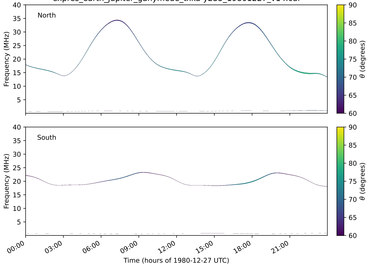
expres_earth_jupiter_ganymede_txka-y235_19801227_v14.cdf
