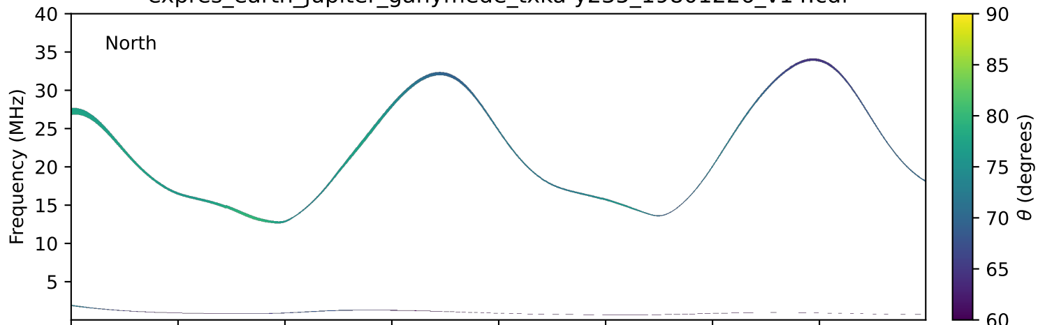
expres_earth_jupiter_ganymede_txka-y235_19801226_v14.cdf
