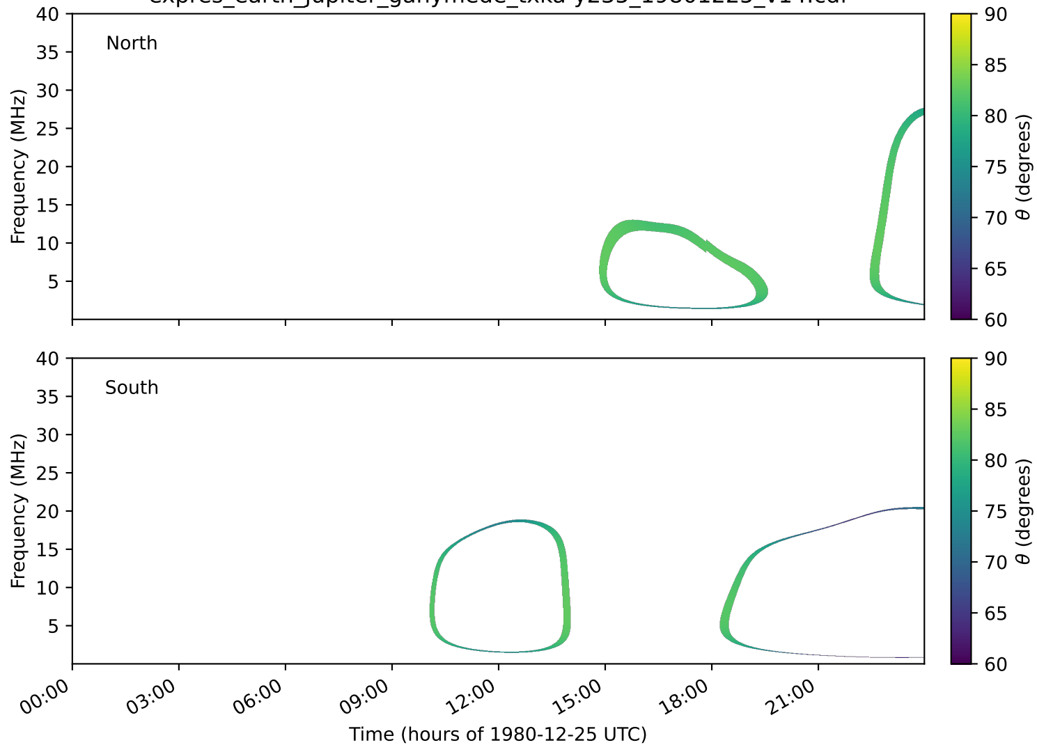
expres_earth_jupiter_ganymede_txka-y235_19801225_v14.cdf
