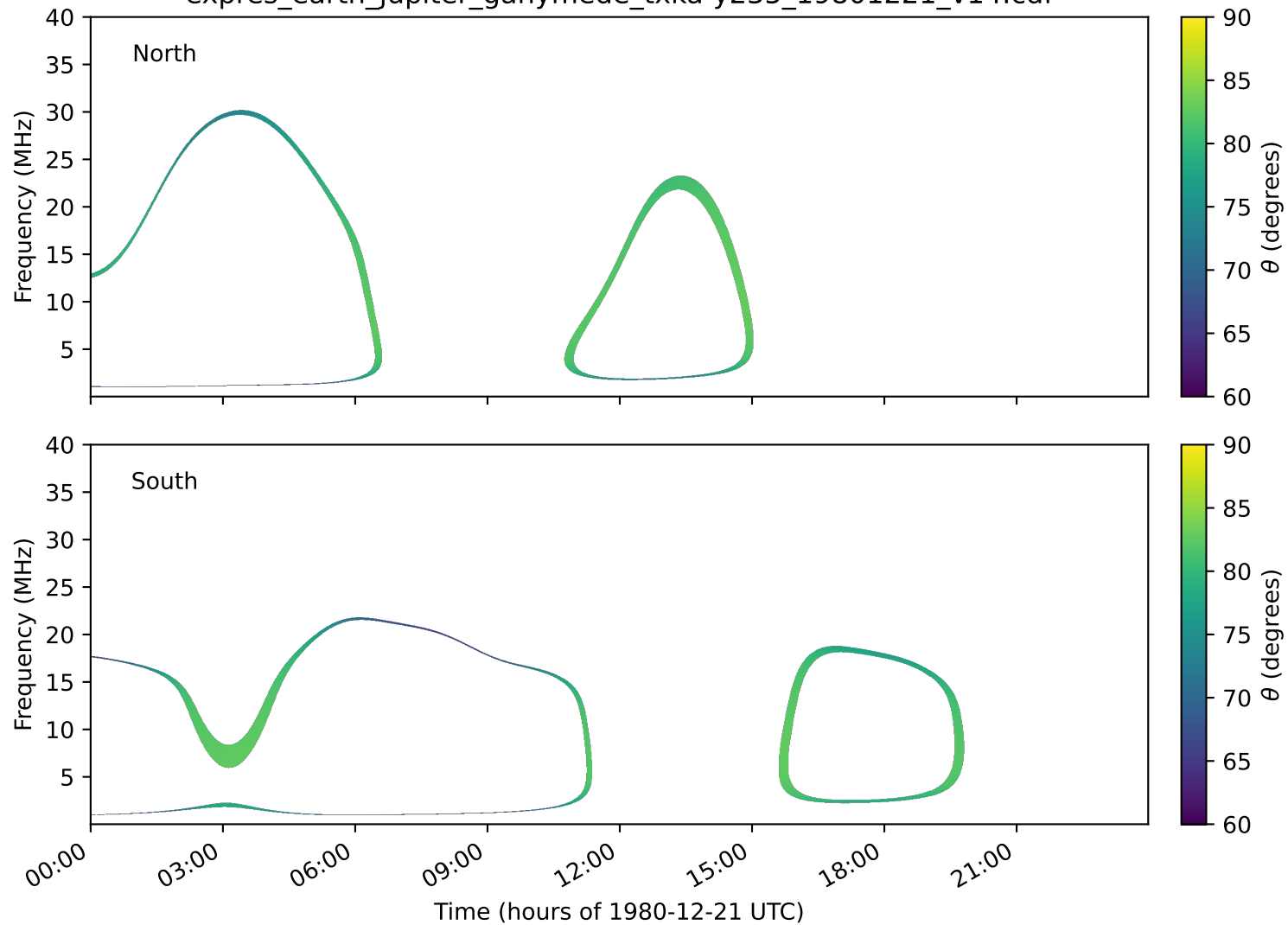
expres_earth_jupiter_ganymede_txka-y235_19801221_v14.cdf
