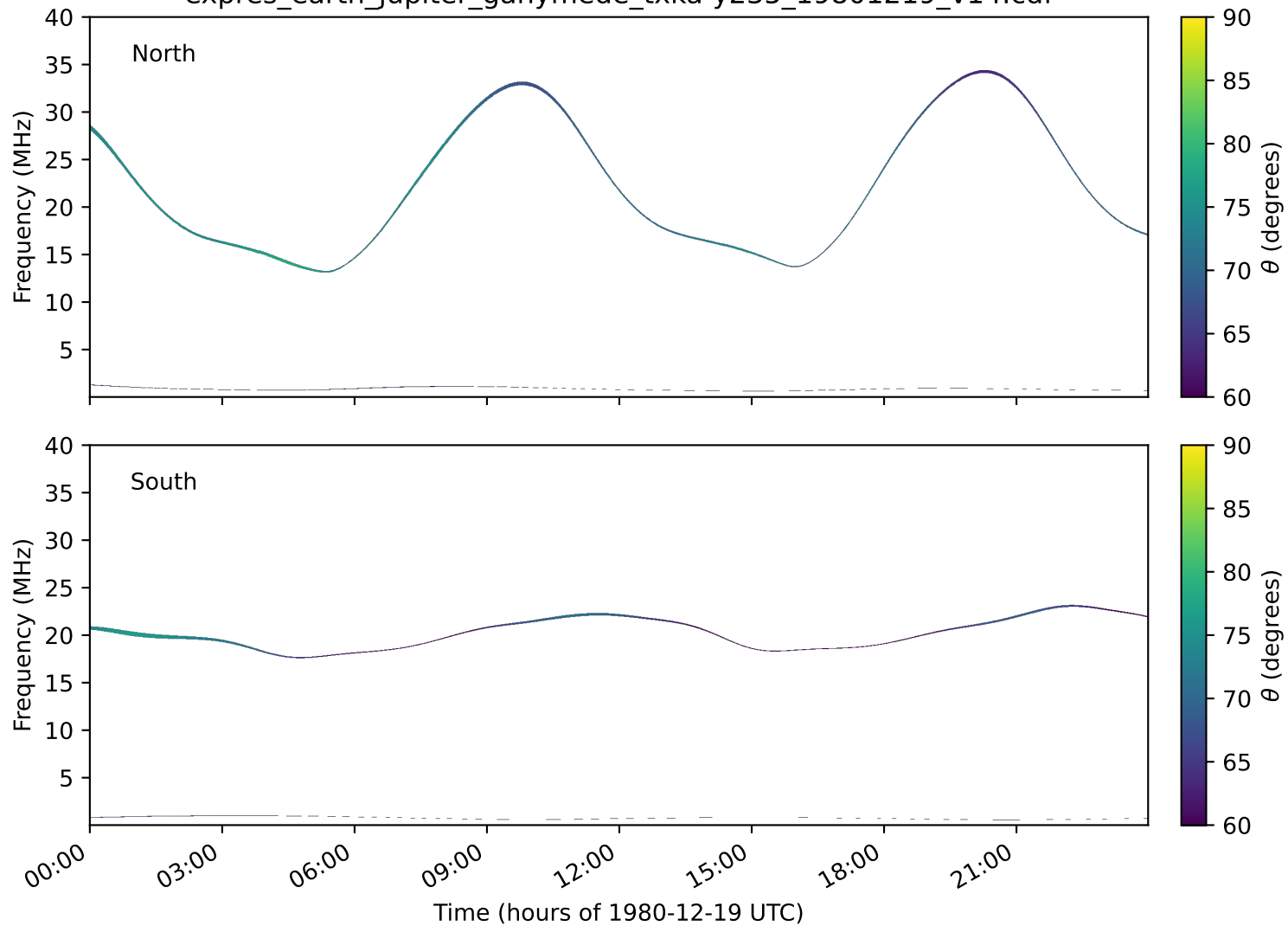
expres_earth_jupiter_ganymede_txka-y235_19801219_v14.cdf
