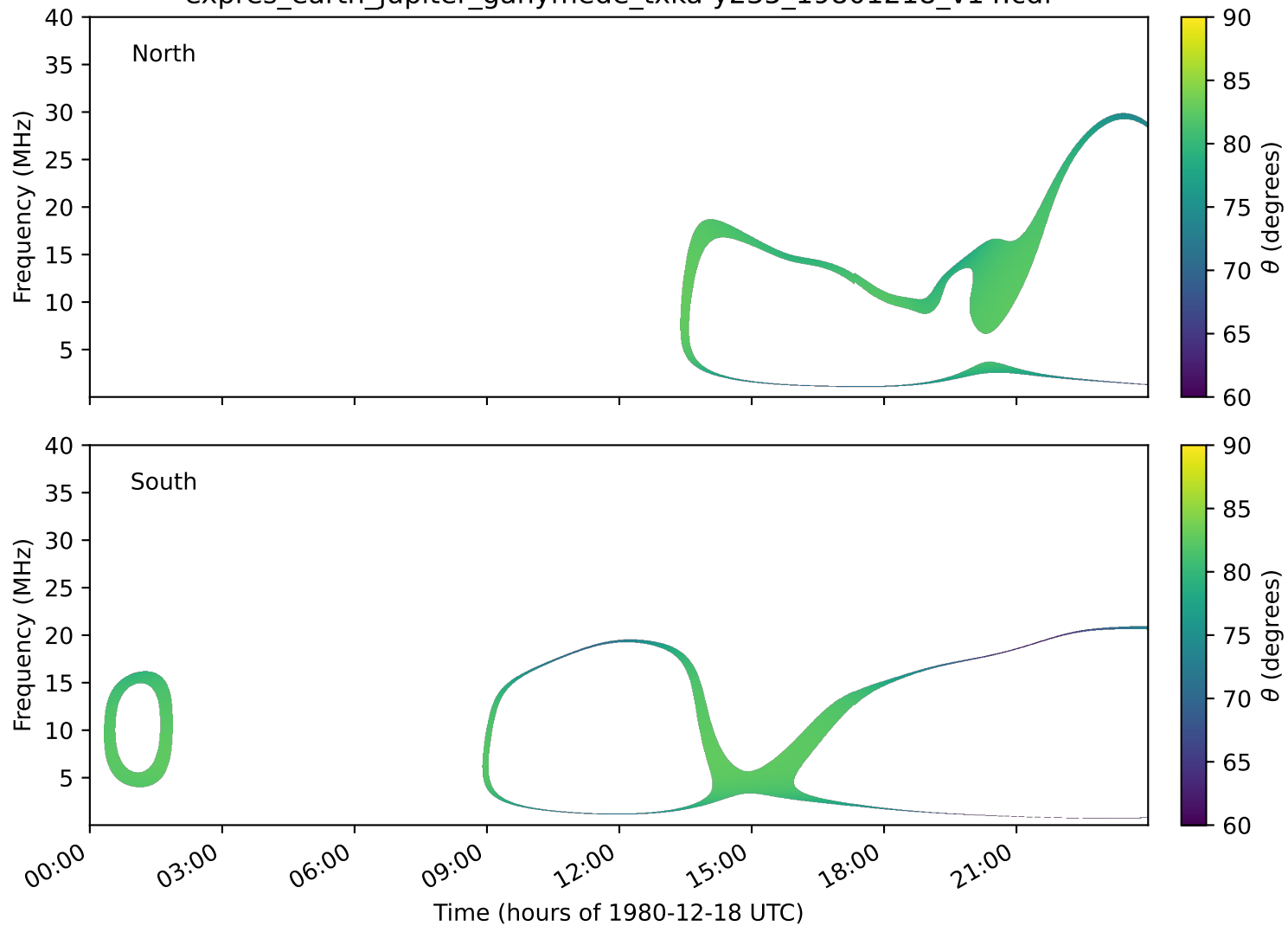
expres_earth_jupiter_ganymede_txka-y235_19801218_v14.cdf
