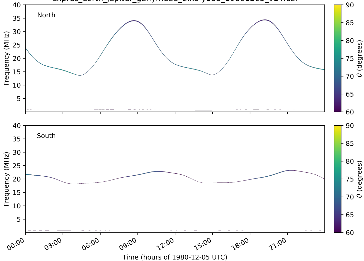
expres_earth_jupiter_ganymede_txka-y235_19801205_v14.cdf
