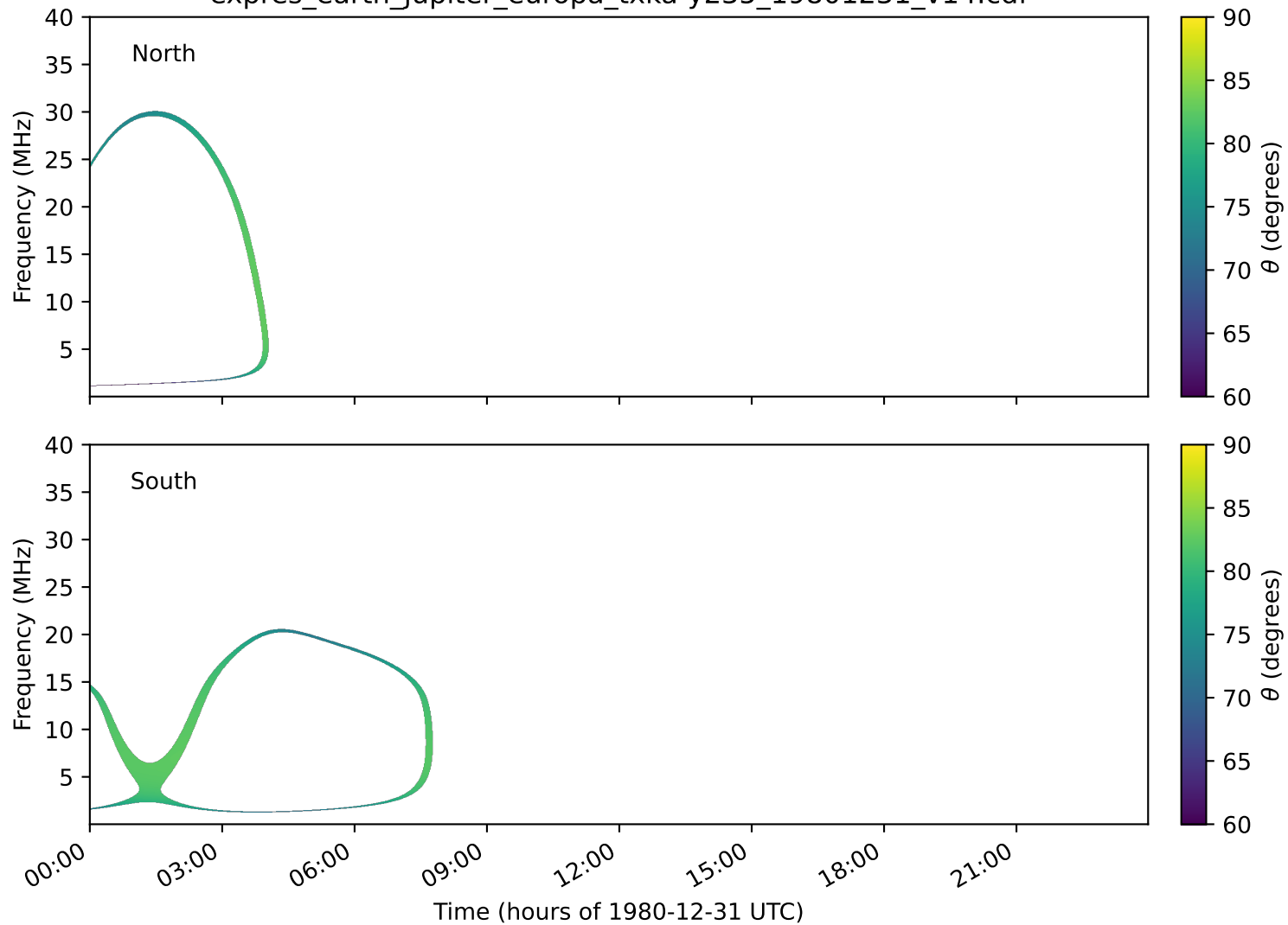
expres_earth_jupiter_europa_txka-y235_19801231_v14.cdf
