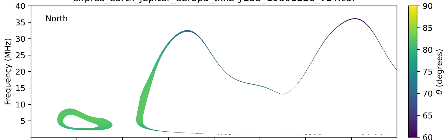
expres_earth_jupiter_europa_txka-y235_19801226_v14.cdf
