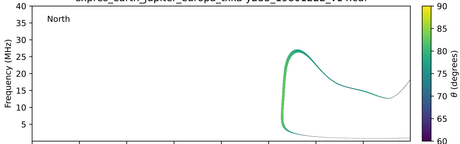
expres_earth_jupiter_europa_txka-y235_19801222_v14.cdf
