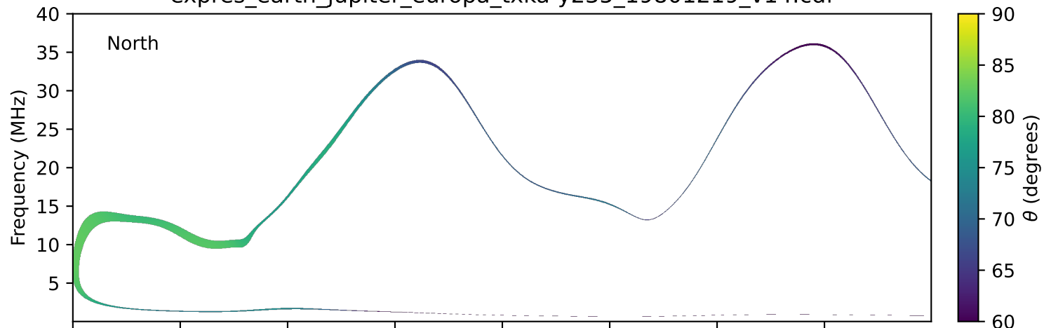
expres_earth_jupiter_europa_txka-y235_19801219_v14.cdf
