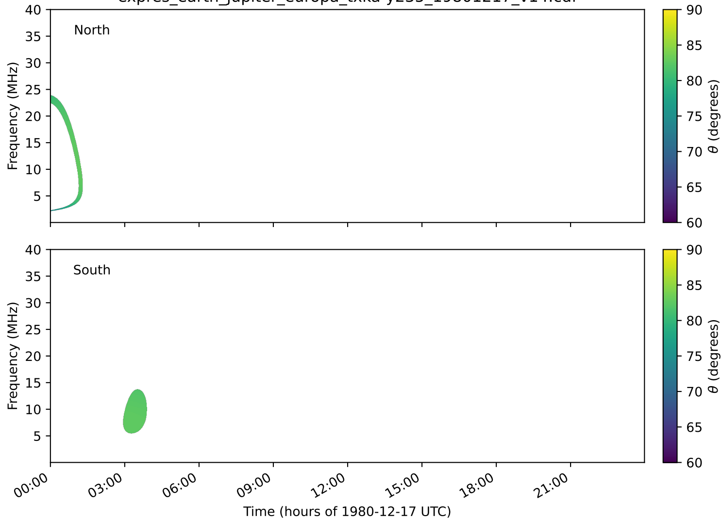
expres_earth_jupiter_europa_txka-y235_19801217_v14.cdf
