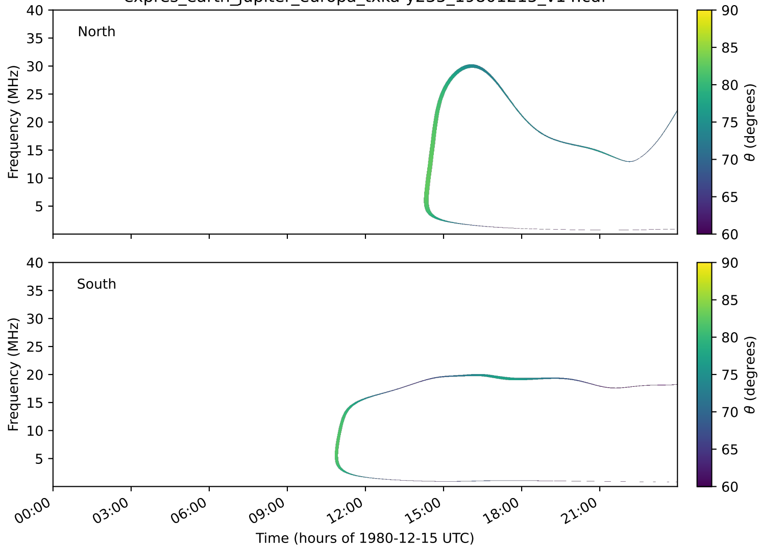
expres_earth_jupiter_europa_txka-y235_19801215_v14.cdf
