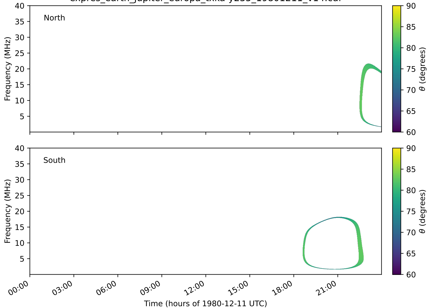
expres_earth_jupiter_europa_txka-y235_19801211_v14.cdf
