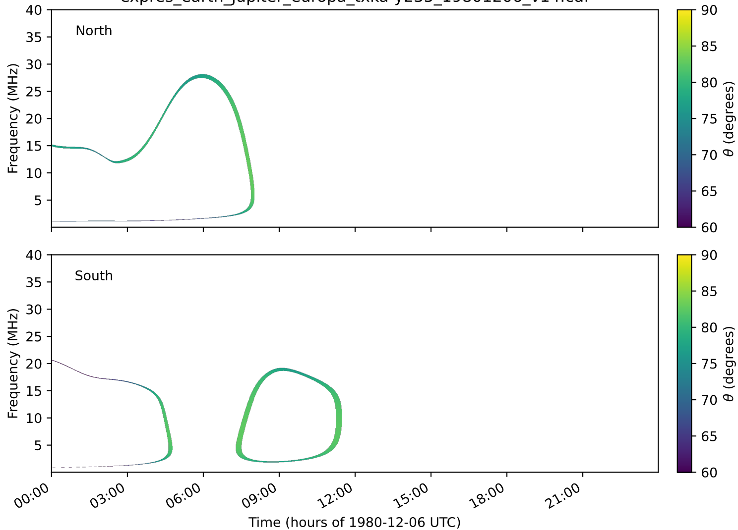
expres_earth_jupiter_europa_txka-y235_19801206_v14.cdf
