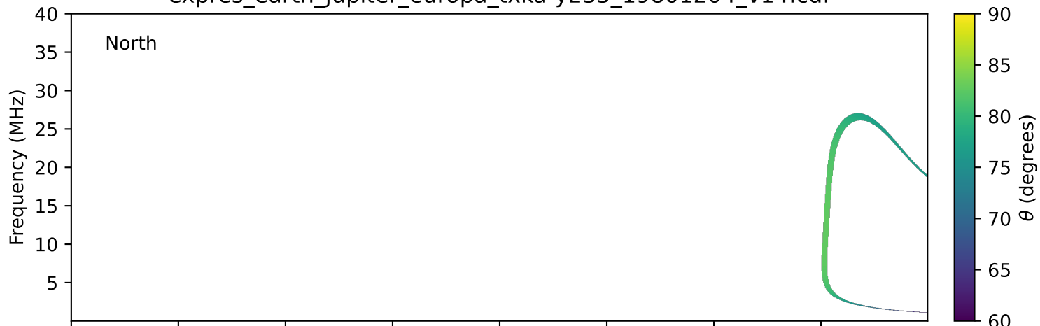
expres_earth_jupiter_europa_txka-y235_19801204_v14.cdf
