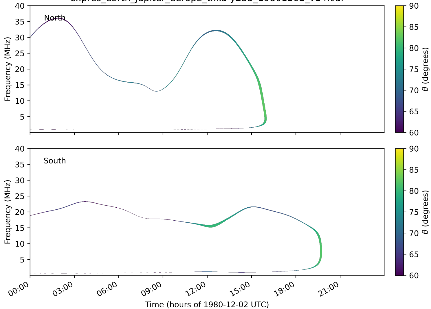
expres_earth_jupiter_europa_txka-y235_19801202_v14.cdf
