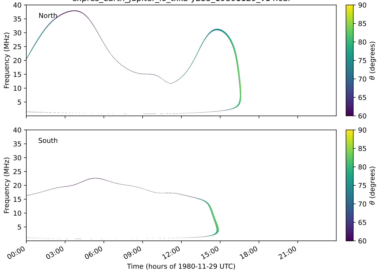
expres_earth_jupiter_io_txka-y235_19801129_v14.cdf
