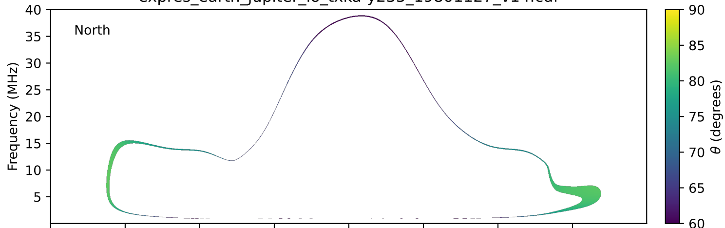
expres_earth_jupiter_io_txka-y235_19801127_v14.cdf
