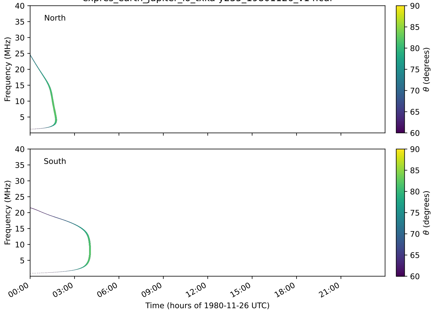
expres_earth_jupiter_io_txka-y235_19801126_v14.cdf
