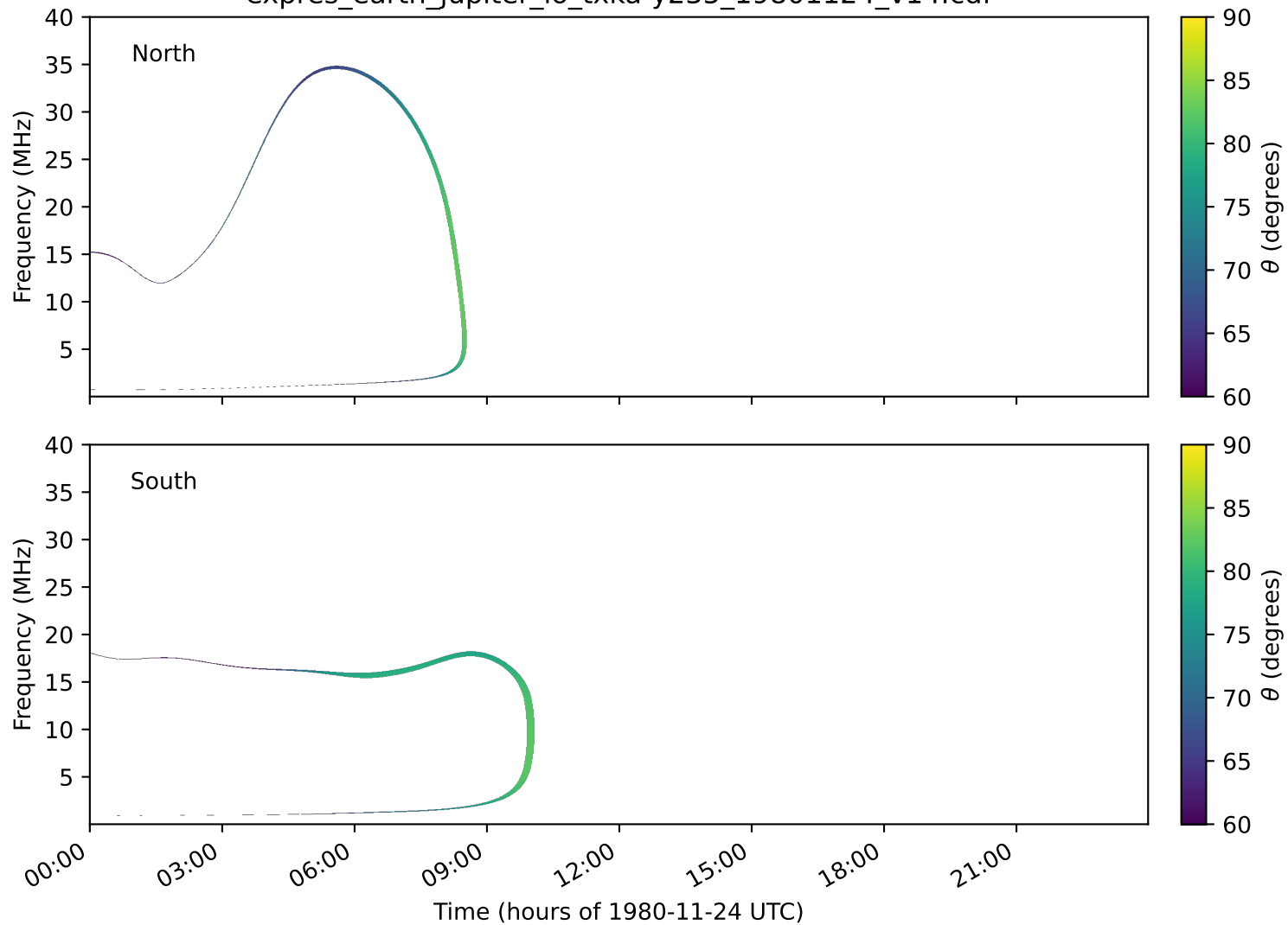
expres_earth_jupiter_io_txka-y235_19801124_v14.cdf
