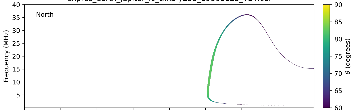
expres_earth_jupiter_io_txka-y235_19801123_v14.cdf
