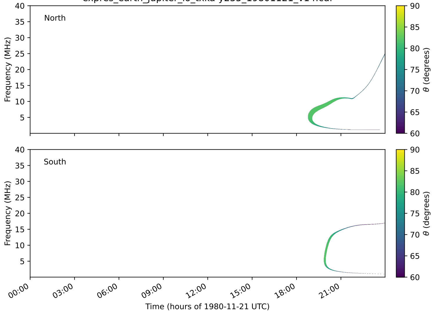
expres_earth_jupiter_io_txka-y235_19801121_v14.cdf
