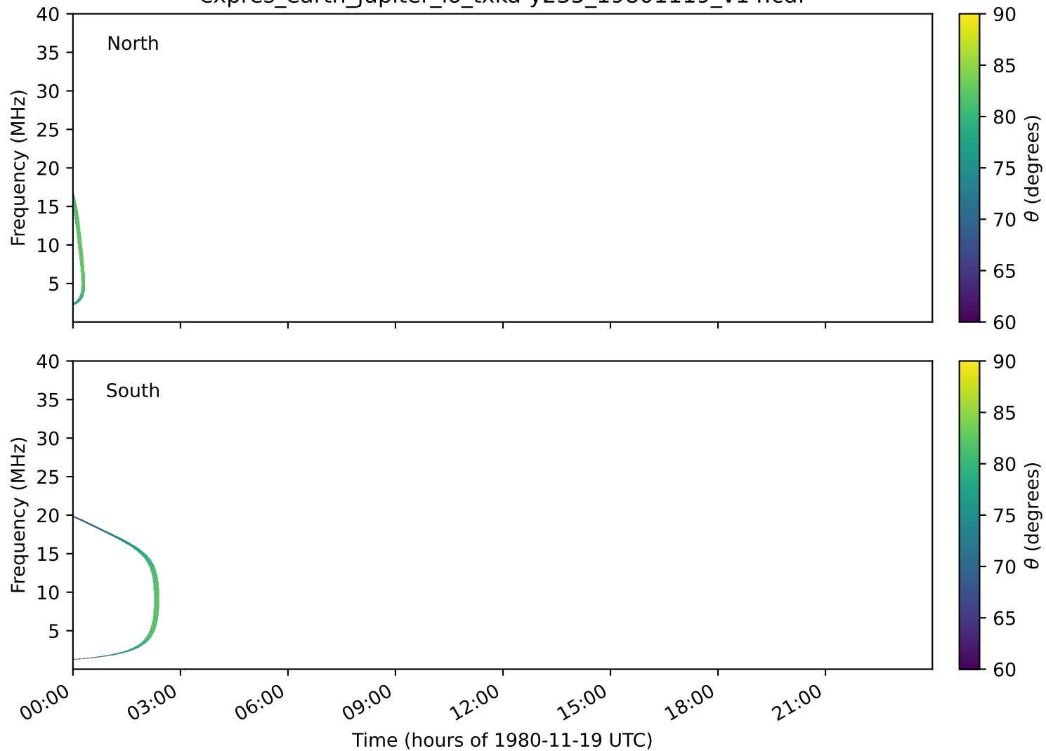
expres_earth_jupiter_io_txka-y235_19801119_v14.cdf
