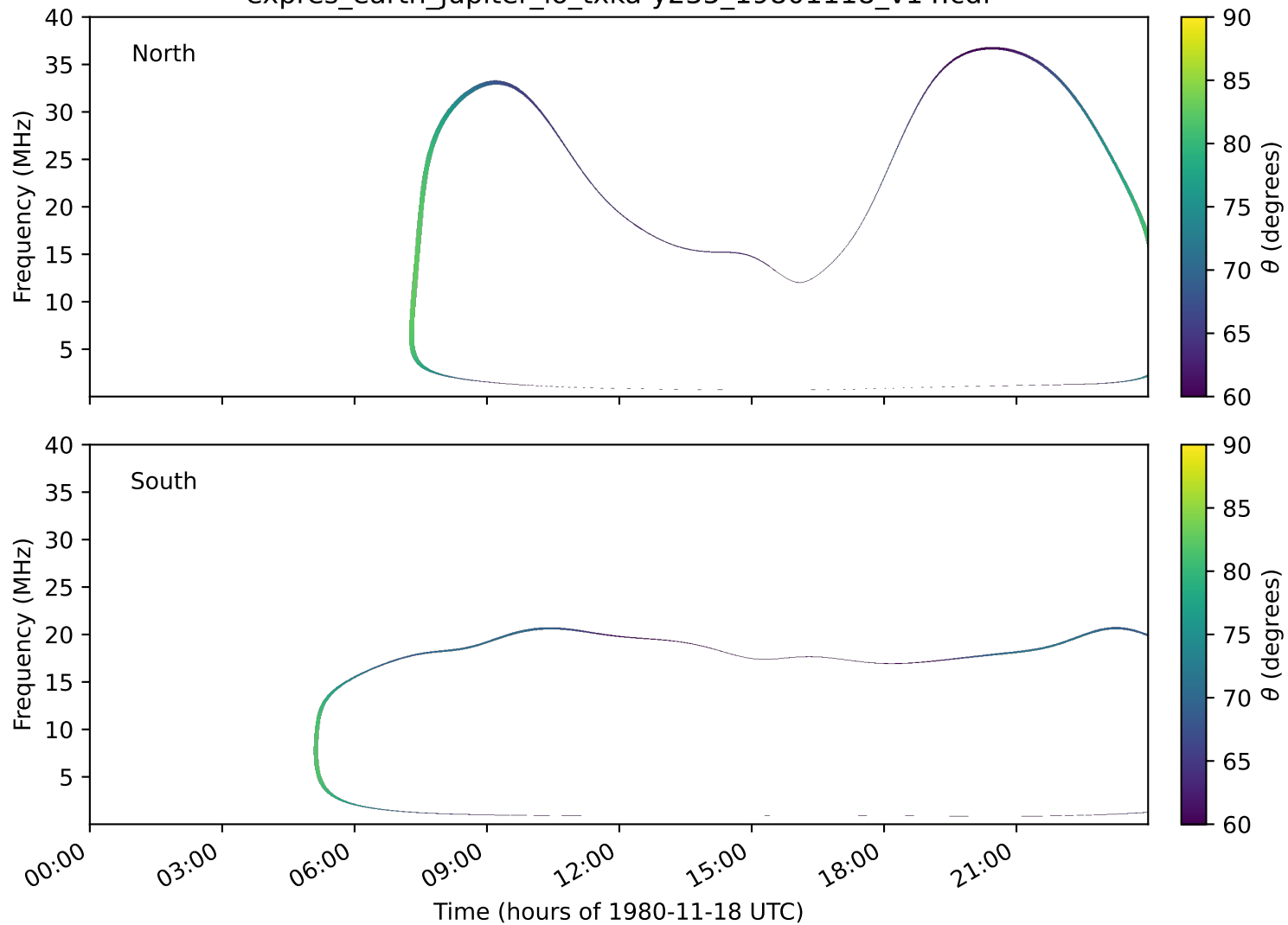
expres_earth_jupiter_io_txka-y235_19801118_v14.cdf
