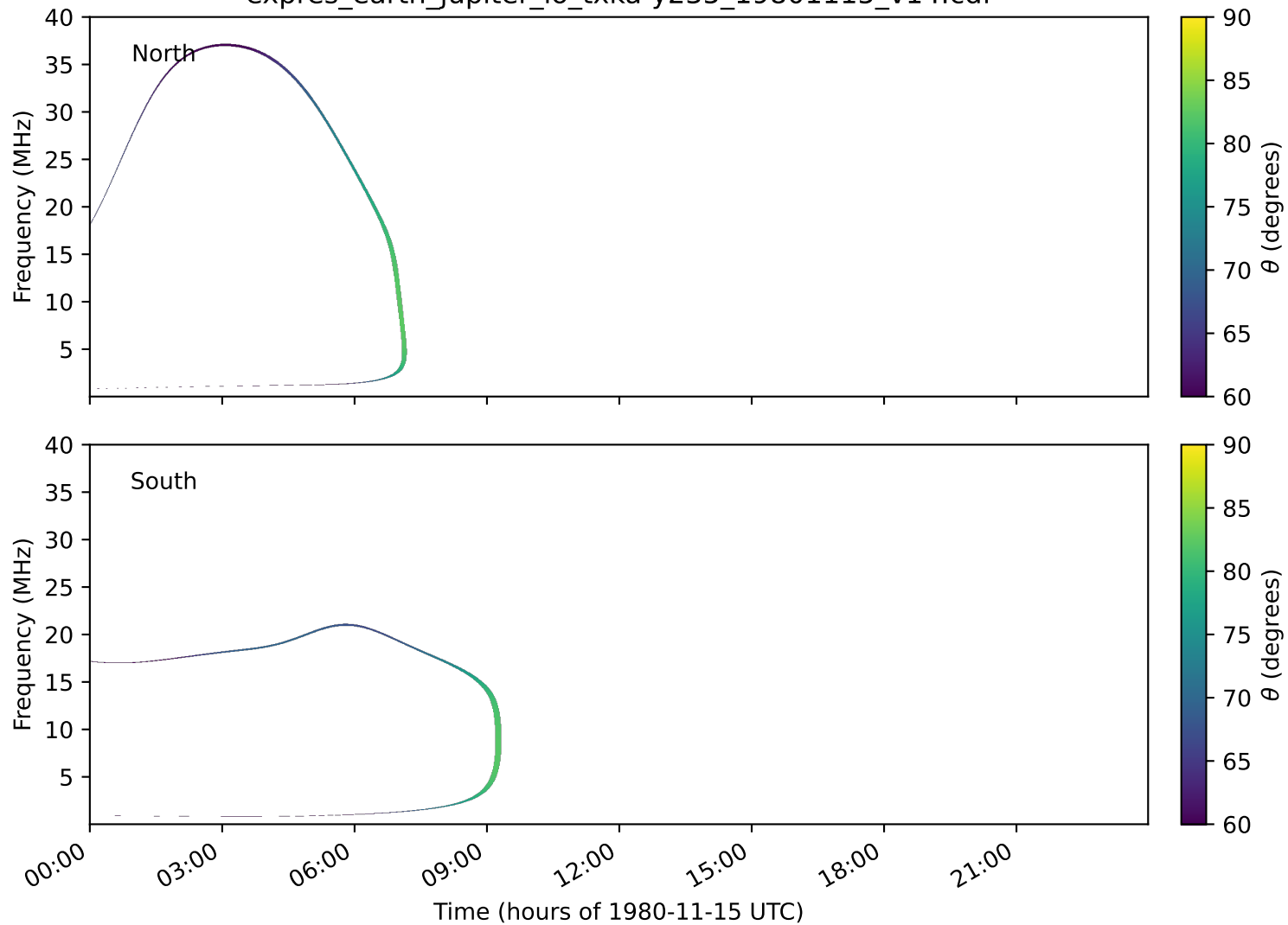
expres_earth_jupiter_io_txka-y235_19801115_v14.cdf
