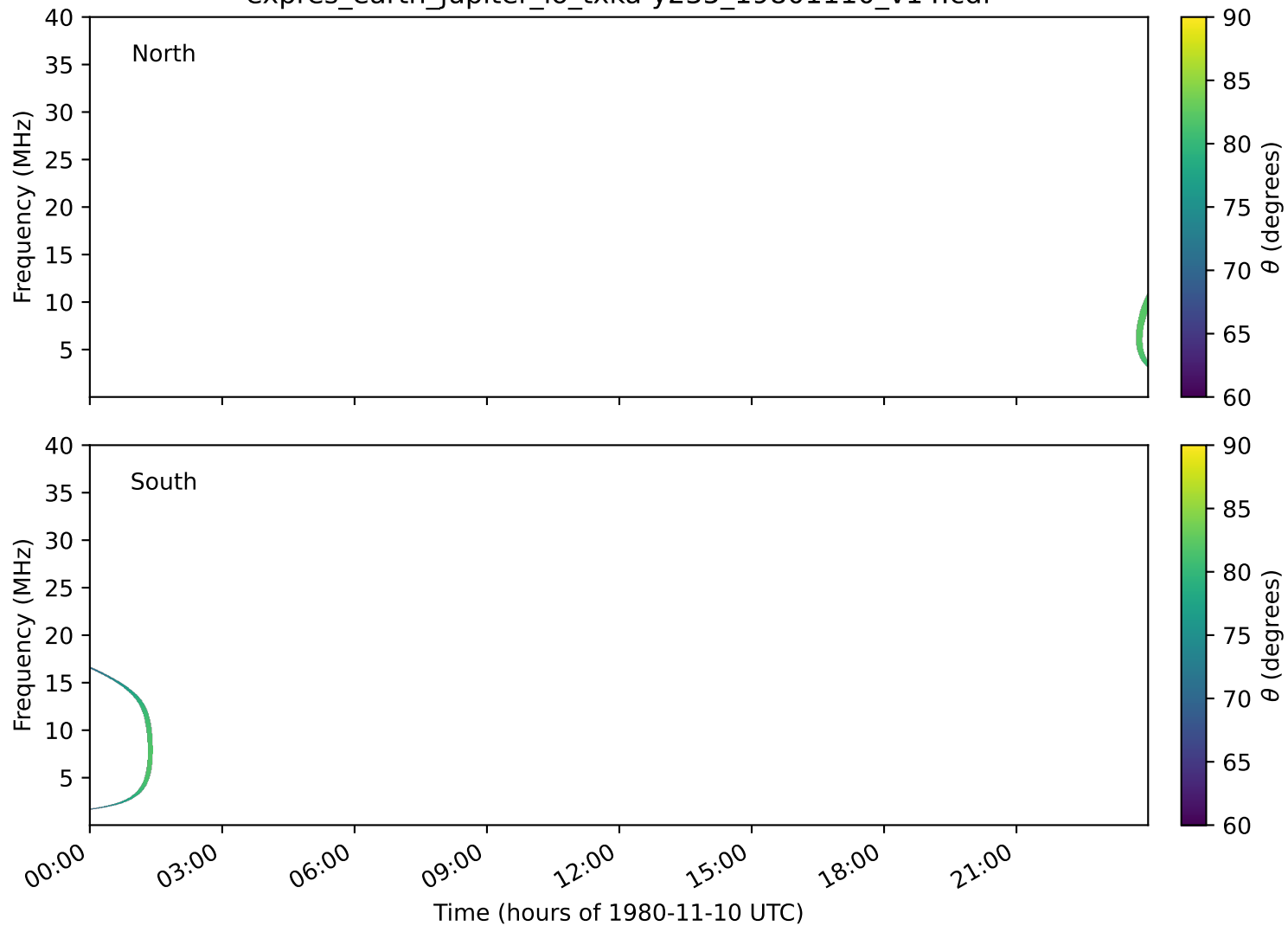
expres_earth_jupiter_io_txka-y235_19801110_v14.cdf
