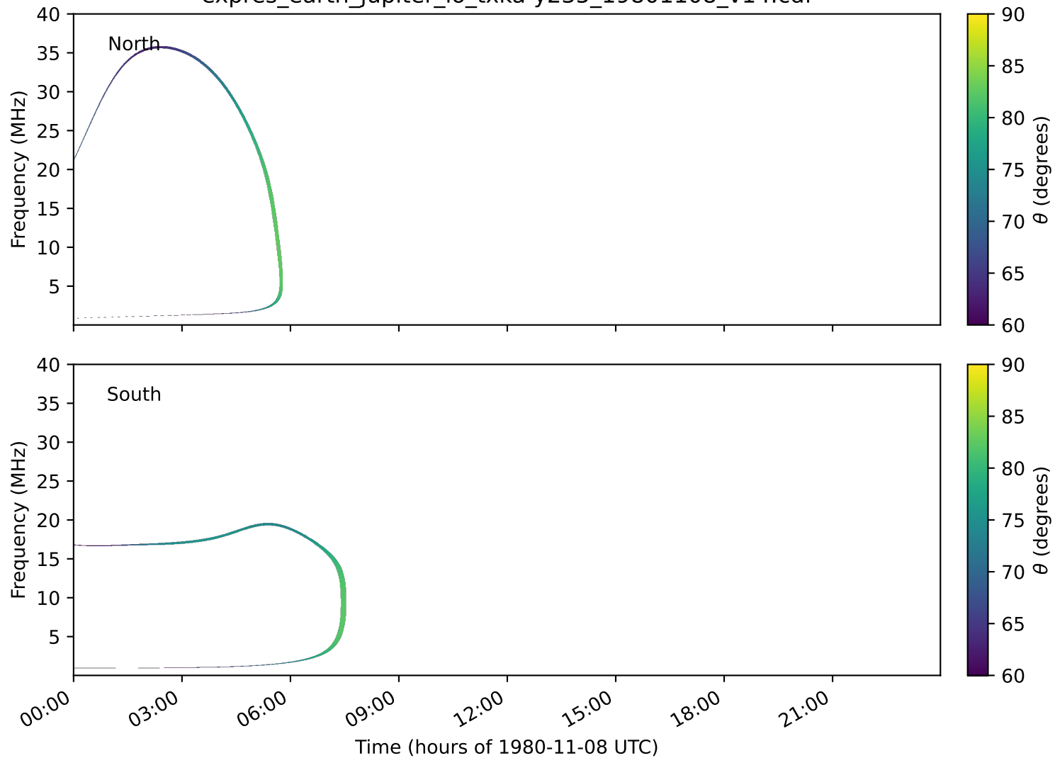
expres_earth_jupiter_io_txka-y235_19801108_v14.cdf
