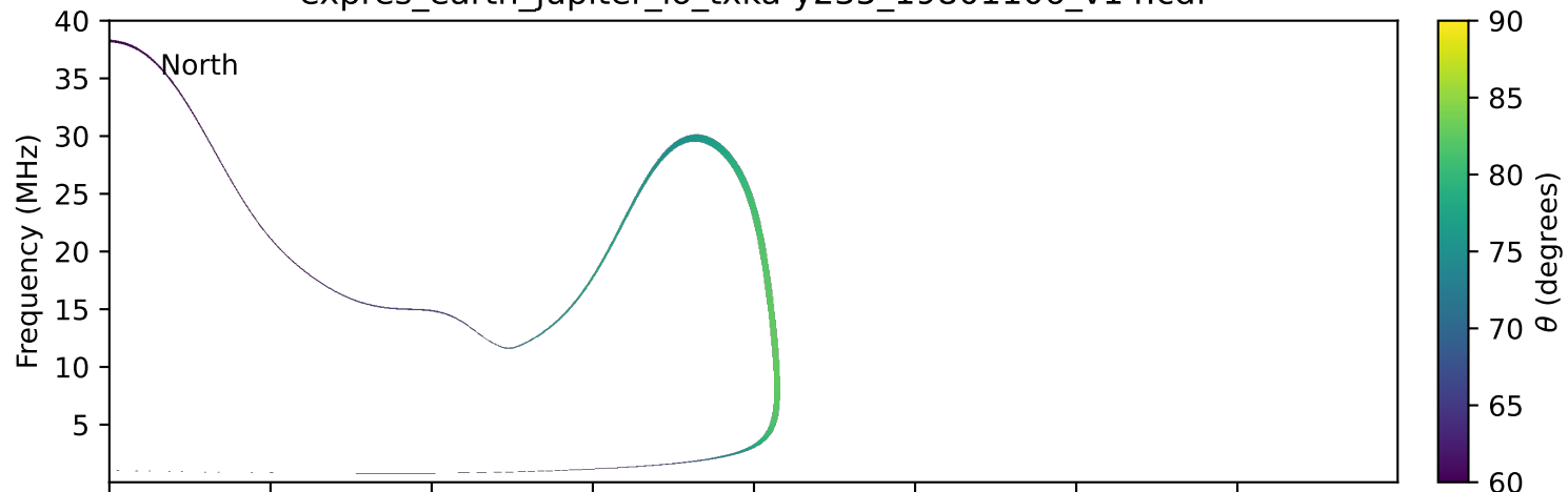
expres_earth_jupiter_io_txka-y235_19801106_v14.cdf
