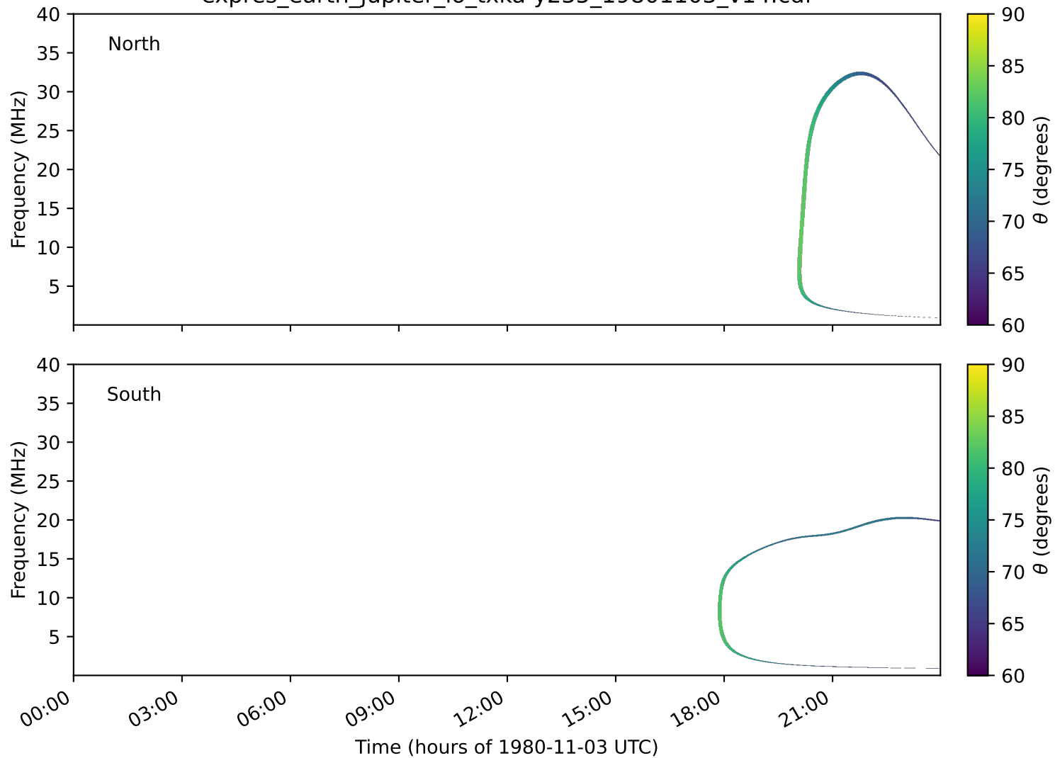
expres_earth_jupiter_io_txka-y235_19801103_v14.cdf
