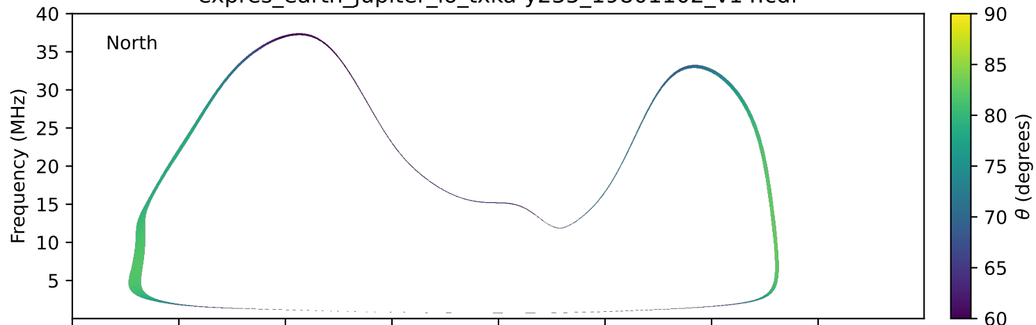
expres_earth_jupiter_io_txka-y235_19801102_v14.cdf
