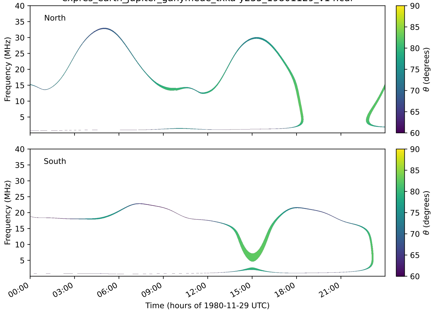
expres_earth_jupiter_ganymede_txka-y235_19801129_v14.cdf
