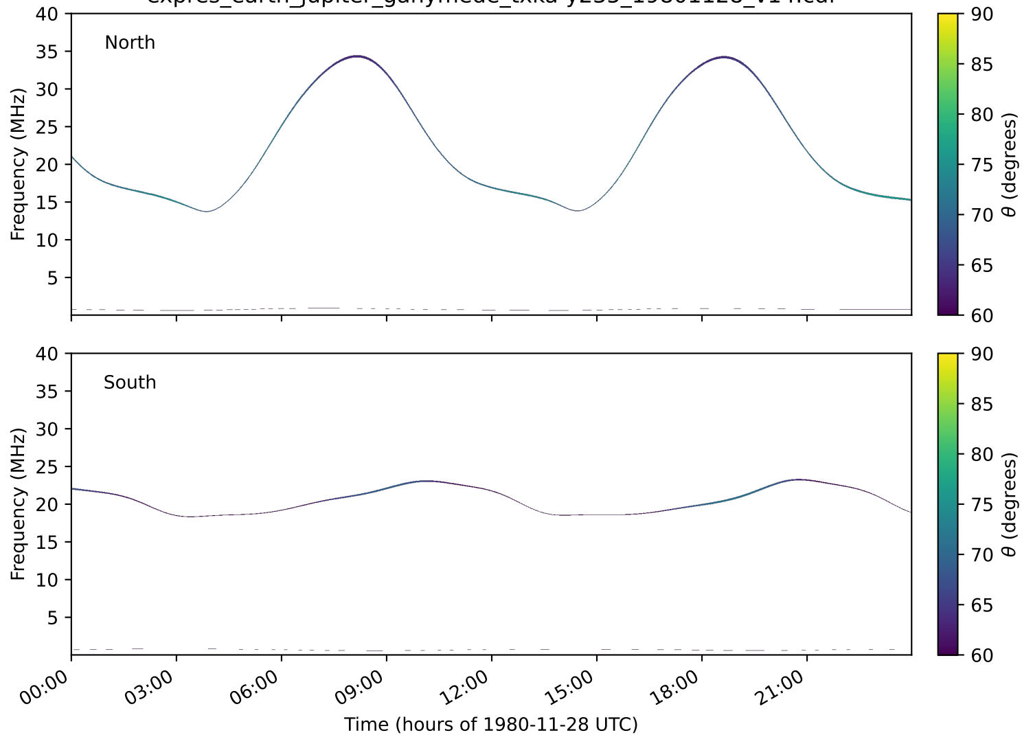
expres_earth_jupiter_ganymede_txka-y235_19801128_v14.cdf
