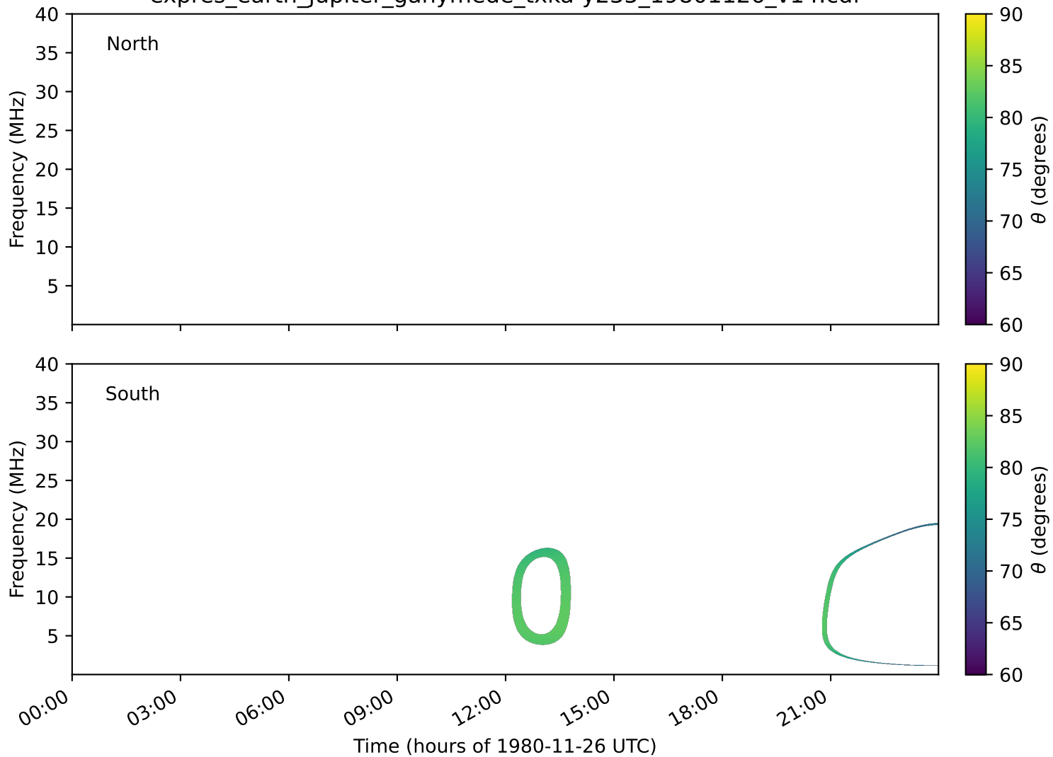
expres_earth_jupiter_ganymede_txka-y235_19801126_v14.cdf
