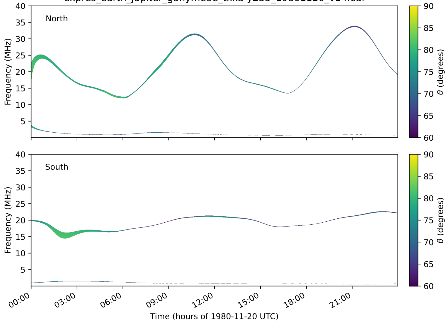
expres_earth_jupiter_ganymede_txka-y235_19801120_v14.cdf
