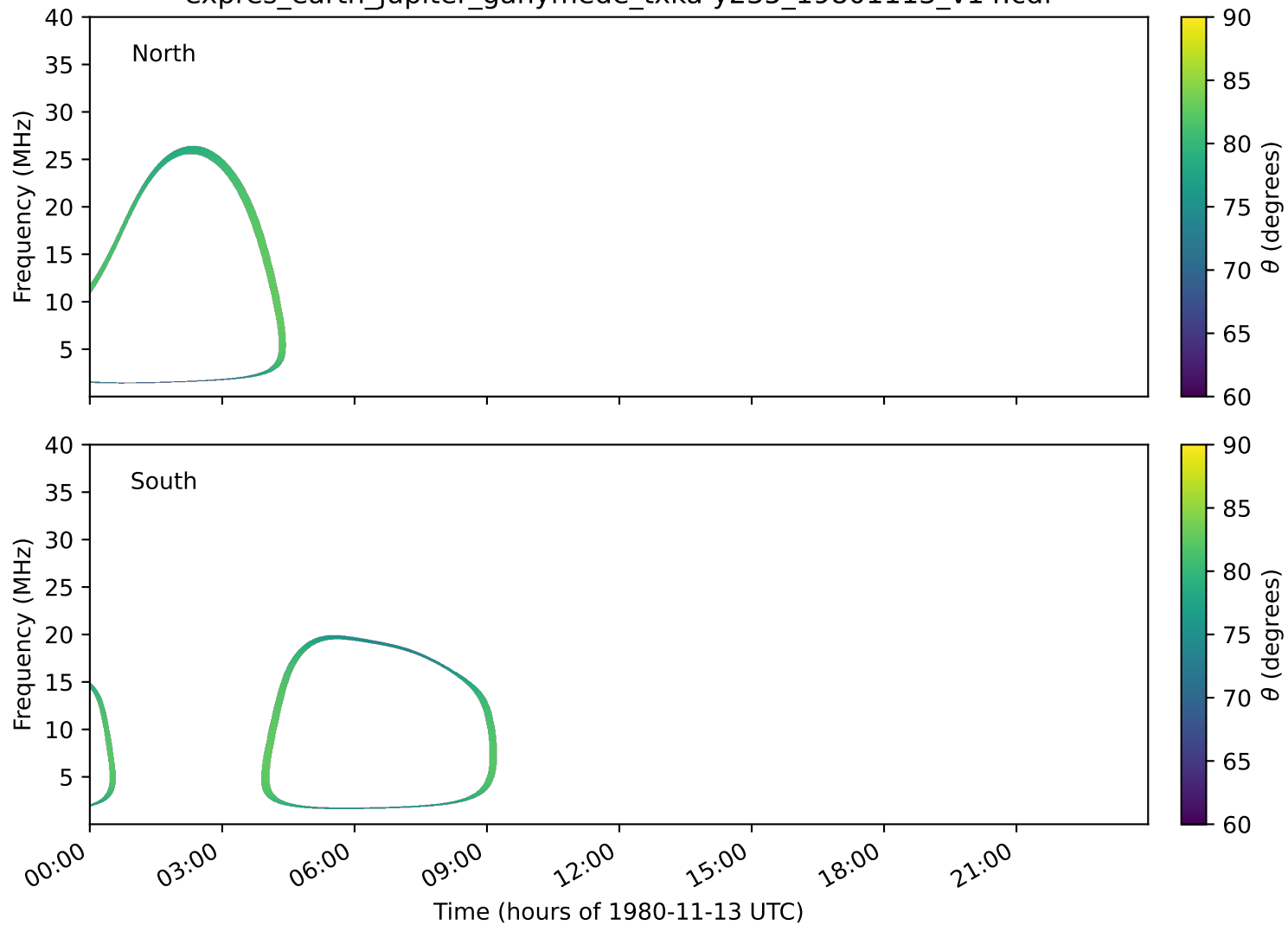
expres_earth_jupiter_ganymede_txka-y235_19801113_v14.cdf
