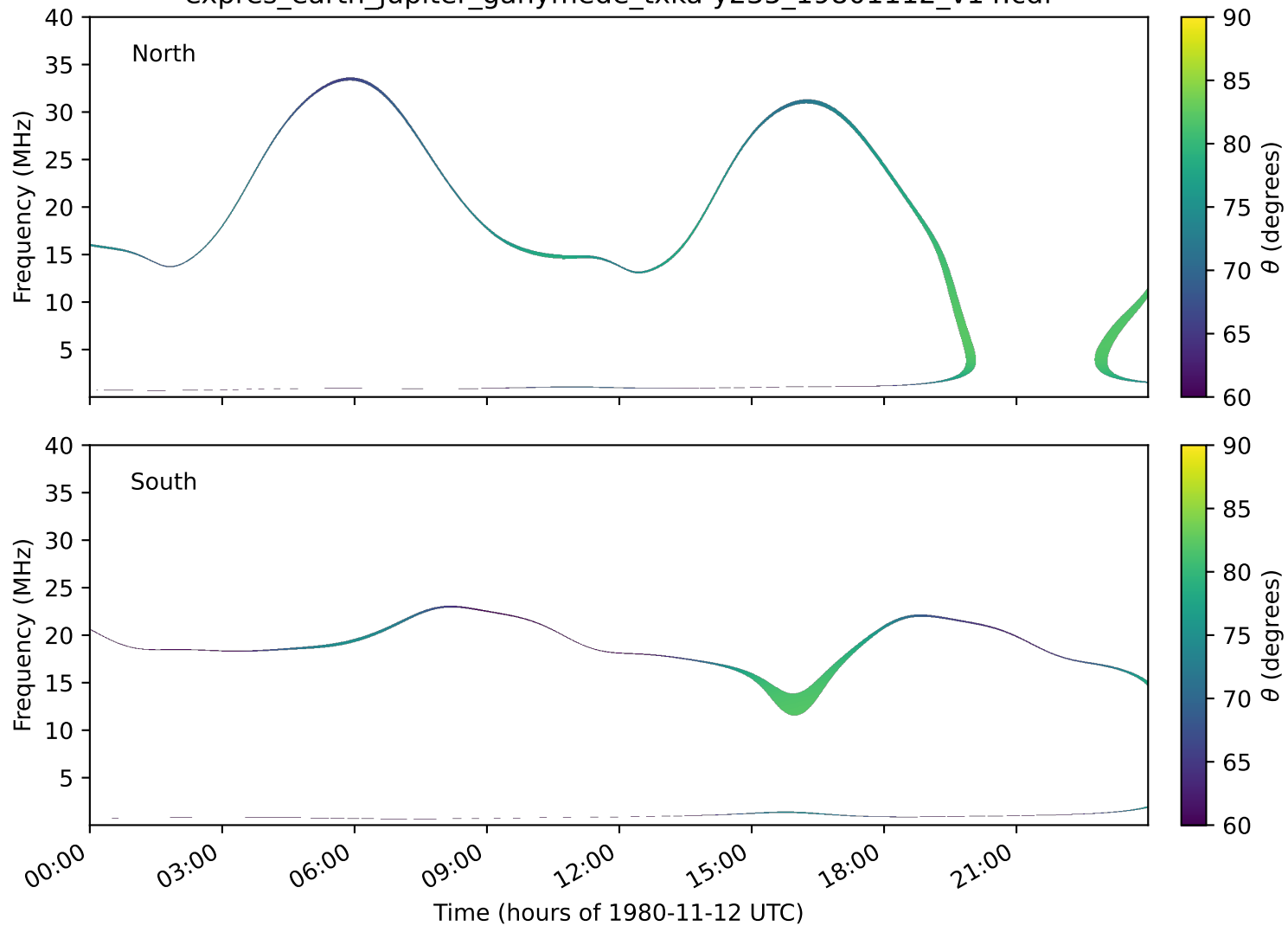
expres_earth_jupiter_ganymede_txka-y235_19801112_v14.cdf
