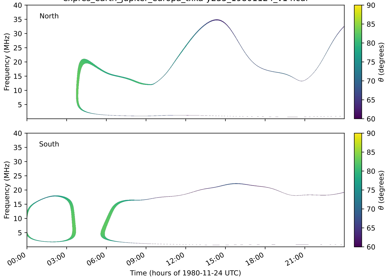
expres_earth_jupiter_europa_txka-y235_19801124_v14.cdf
