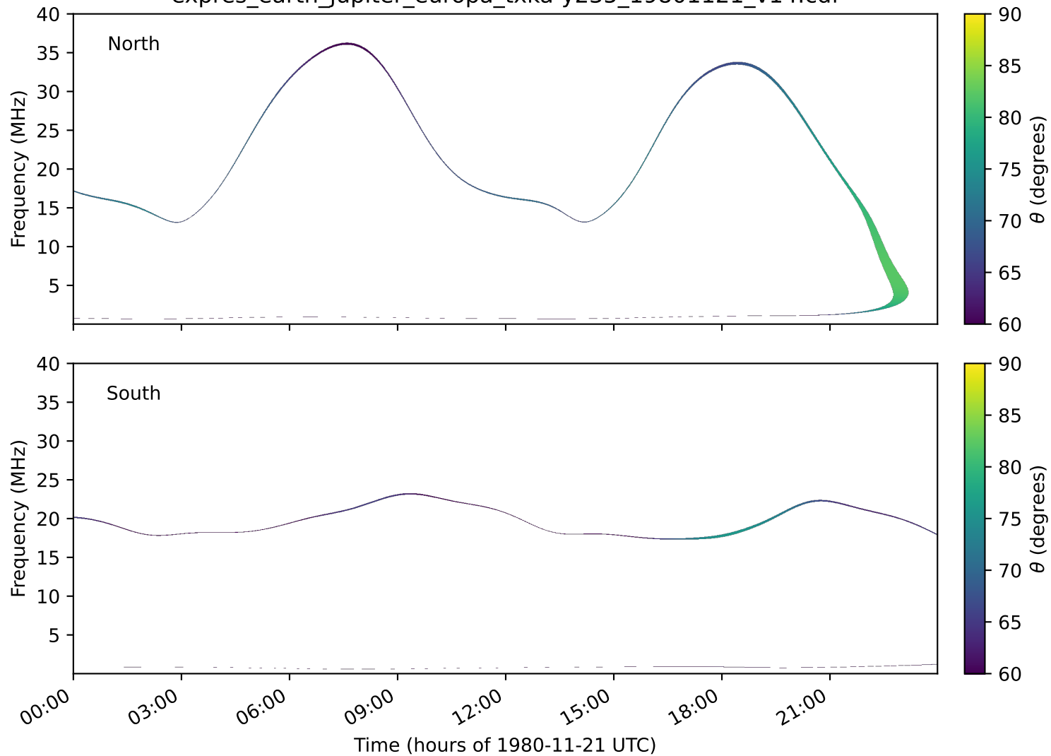
expres_earth_jupiter_europa_txka-y235_19801121_v14.cdf
