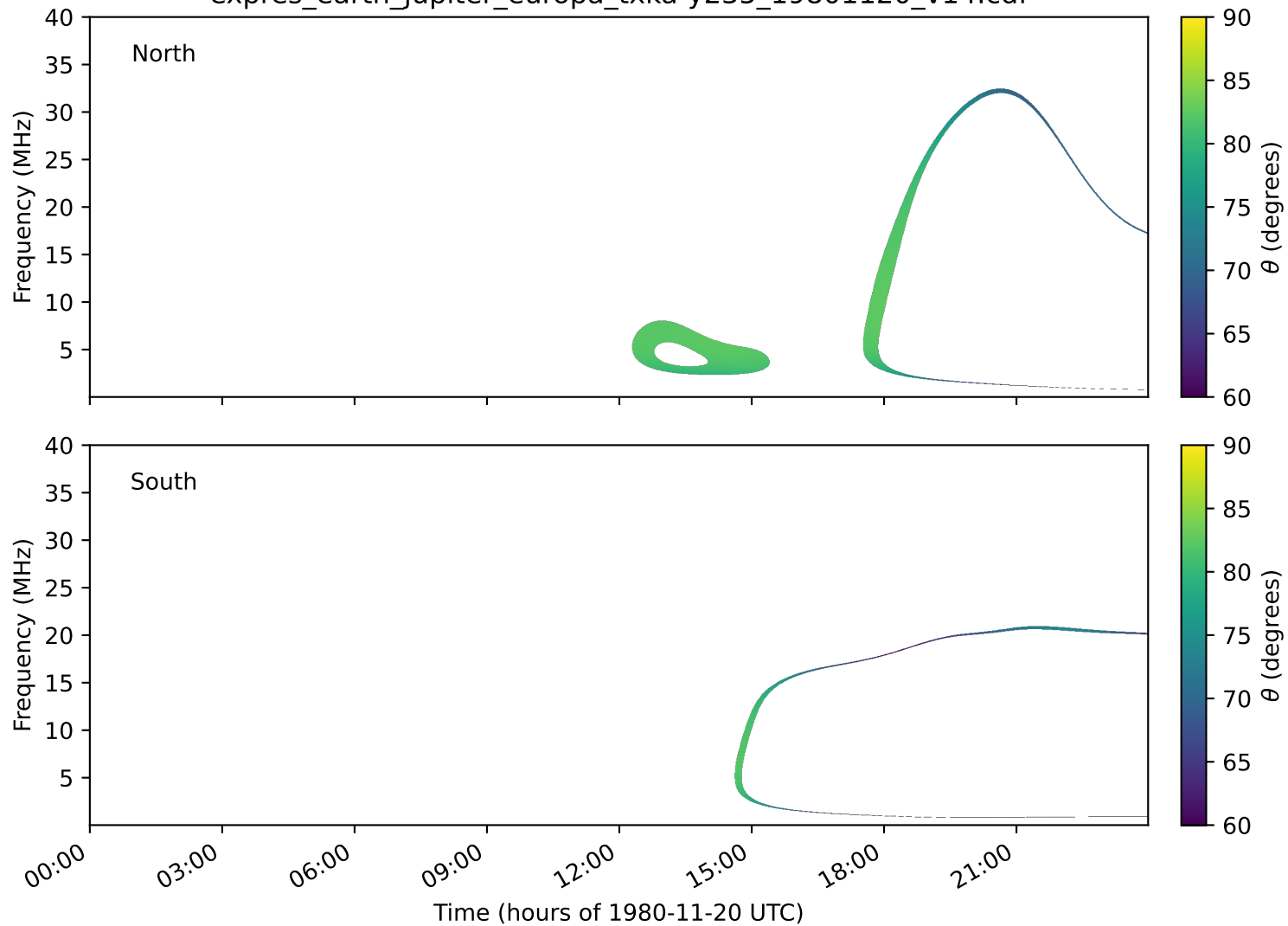
expres_earth_jupiter_europa_txka-y235_19801120_v14.cdf
