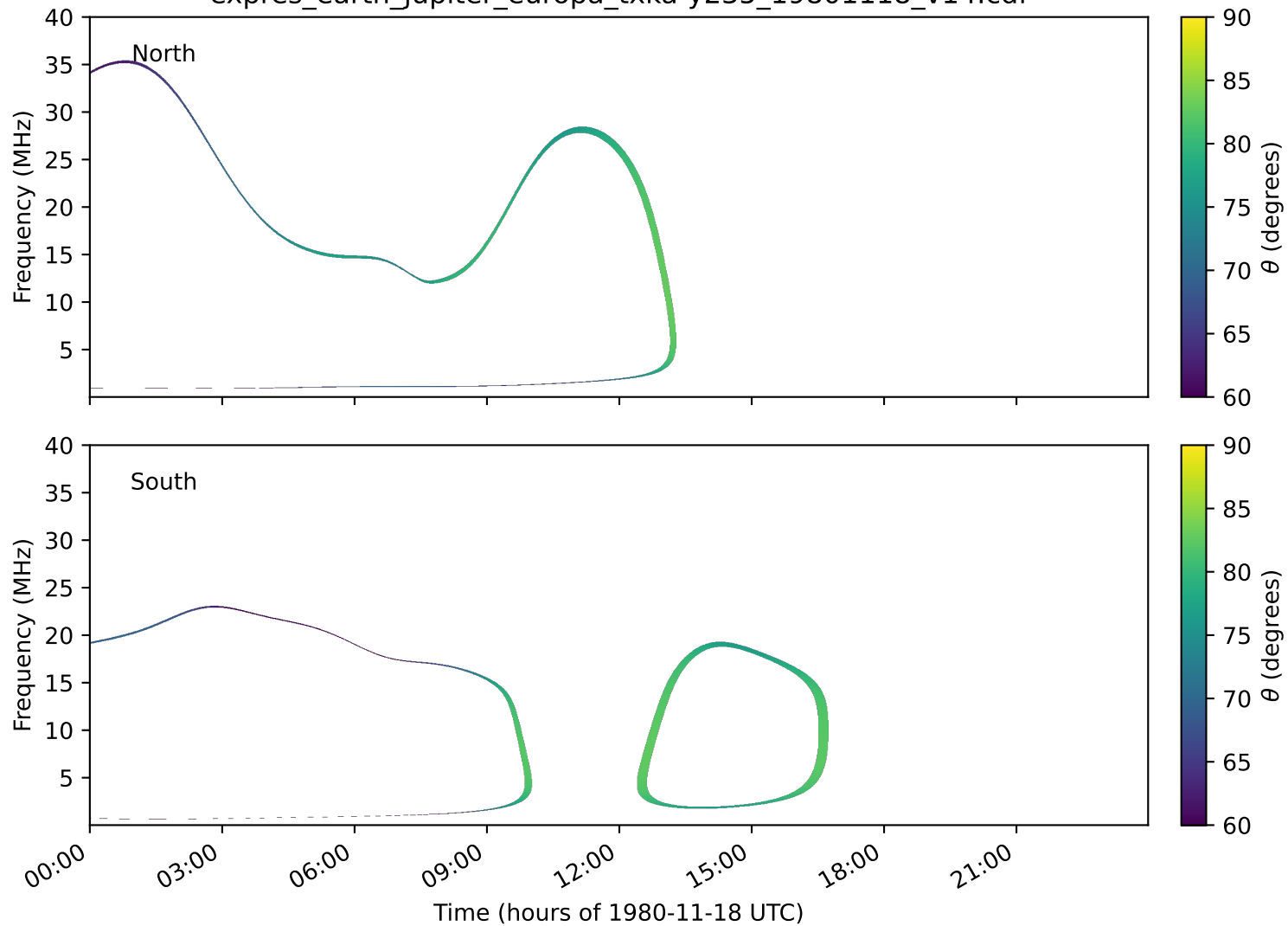
expres_earth_jupiter_europa_txka-y235_19801118_v14.cdf
