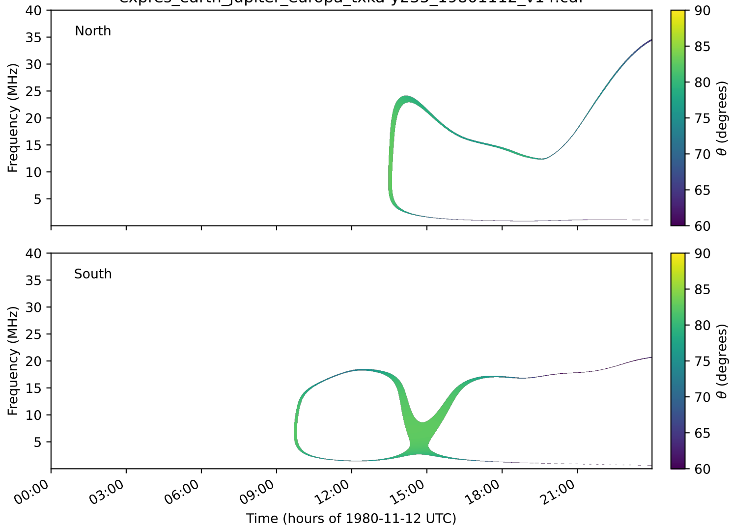
expres_earth_jupiter_europa_txka-y235_19801112_v14.cdf
