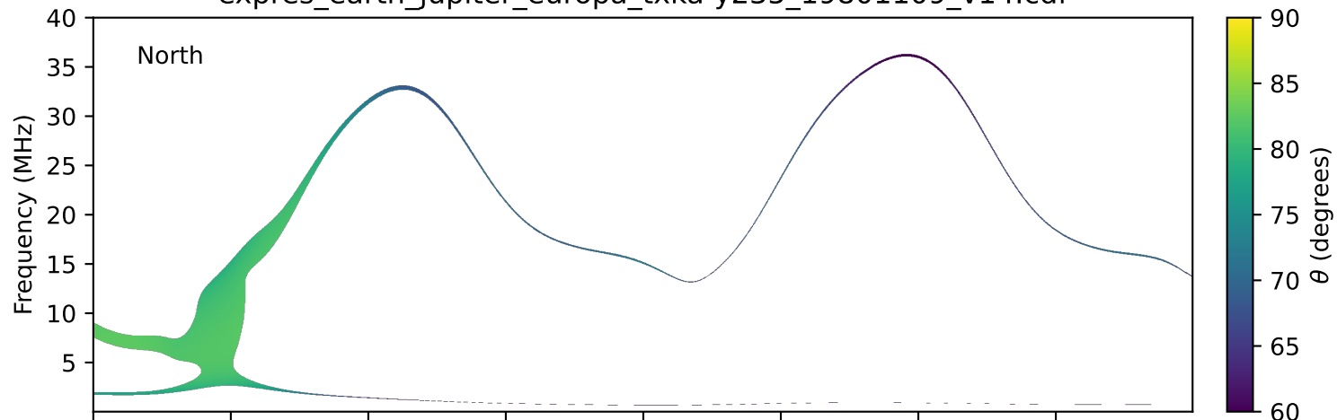
expres_earth_jupiter_europa_txka-y235_19801109_v14.cdf
