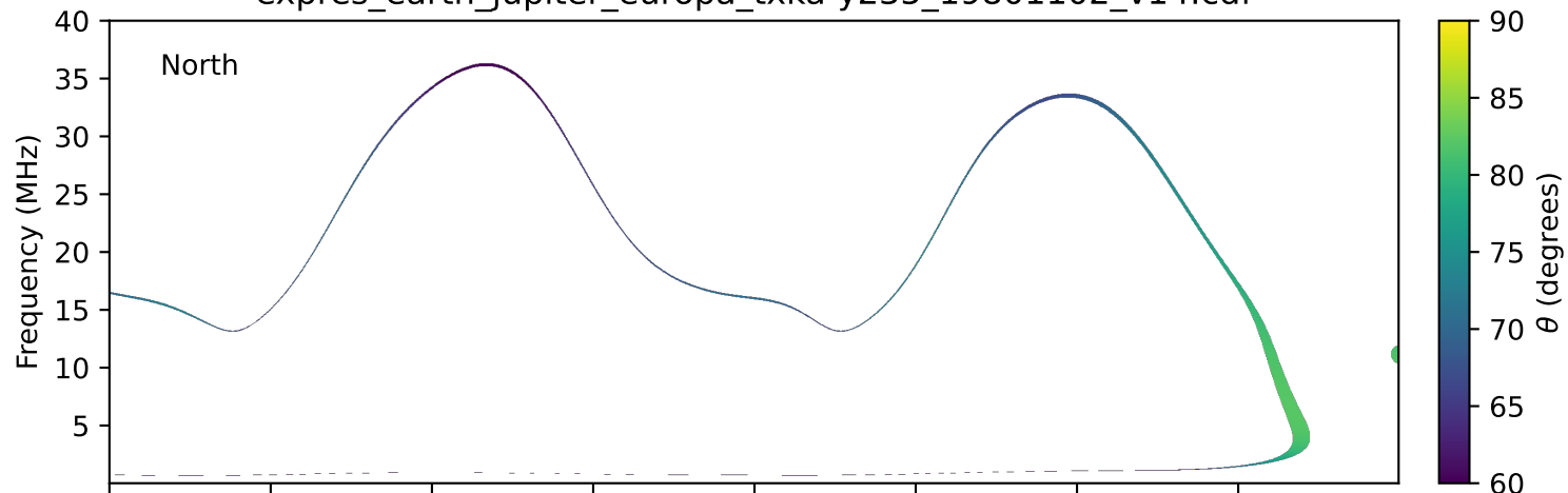
expres_earth_jupiter_europa_txka-y235_19801102_v14.cdf
